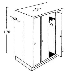
⑪ Narrow locker
